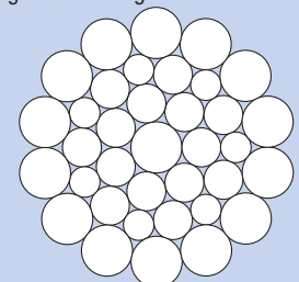
Fig. 12: Warrington-Seale
