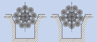
Fig. 18: 9-strand rope in 105° U-groove
