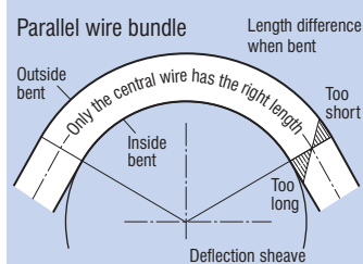
Fig. 3: Rope running over a sheave
