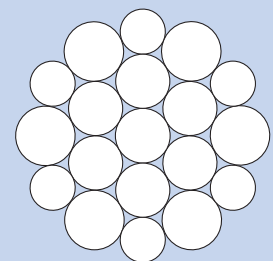
Fig. 10: Warrington
