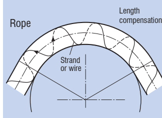
Fig. 3: Rope running over a sheave
