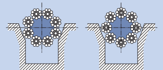
Fig. 17: 8-strand rope in 105° U-groove
