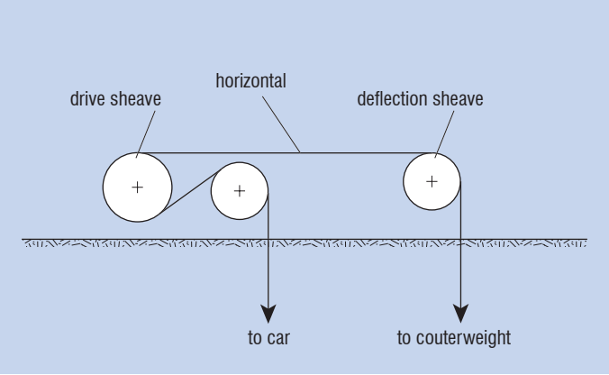
Fig. 36: The laterally positioned machine
