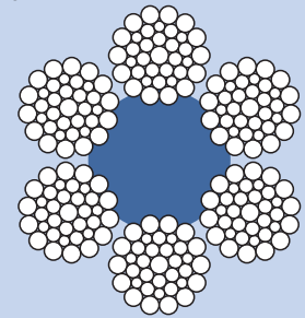
Fig 25: 6x36WS + NFC
