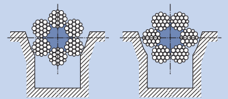
Fig. 16: 6-strand rope in 105° U-groove
